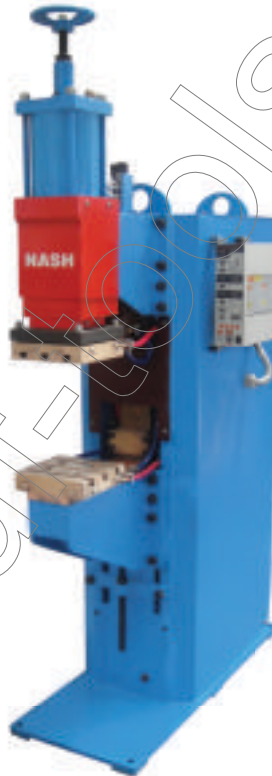
100 KVA Bold Series Projection Welder
